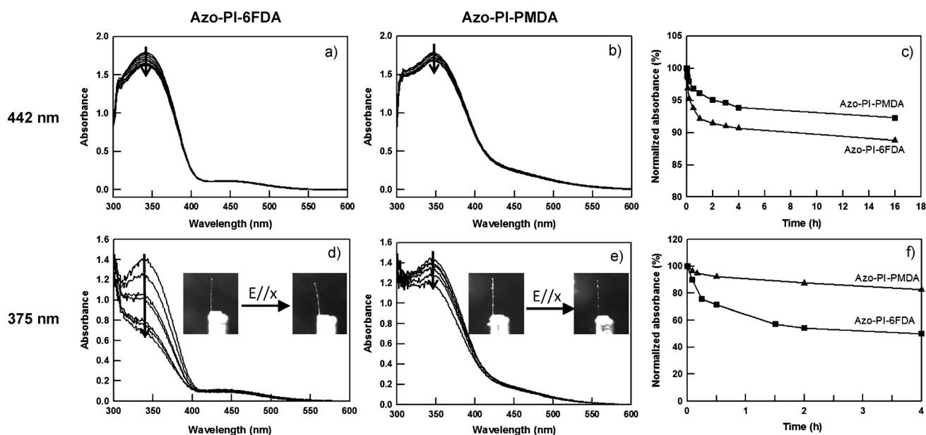
Figure 3. Absorption spectra of azo-PI-6FDA (a) and azo-PI-PMDA (b) during continuous irradiation at 100 mW cm -2 of \lambda = 442 nm light. c) The peak absorbance of the two materials is plotted as a function of irradiation time. Absorption spectra of azo-PI-6FDA (d) and azo-PI-PMDA (e) during continuous irradiation at 50 mW cm -2 of \lambda = 375 nm light. f) The peak absorbance of the two materials is plotted as a function of irradiation time.
